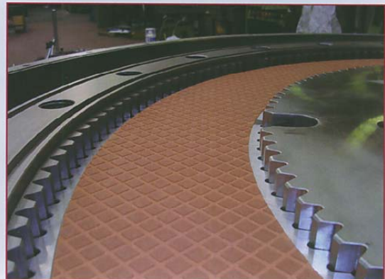
Friction material in the disc pack
